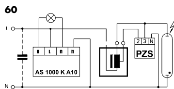
Start-up switch for standard HS lamps
