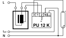
Disconnected control phase (L ST = 0 V) with ballasts with two tapping points
