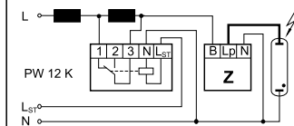
Switching to reduced power using additional impedance (second ballast)
