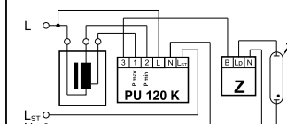
Switching to reduced power using a switchable ballast (ballast with tapping points)
