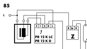
Electronic power reduction without control phase
