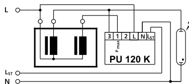
Disconnected control phase (L ST = 0 V) with two ballasts connected in parallel
