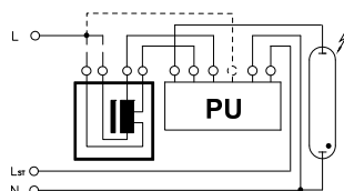
Ballasts with two tapping points and two voltage tapping points (L ST = 0 V or L ST > 0 V)
