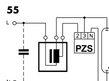
Pulse ignition of standard HS lamps
