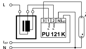
Connected control phase (L ST = 230 V) with ballasts with two tapping points
