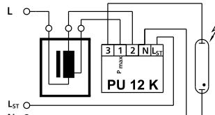
Connected control phase (L ST = 230 V) with ballasts with two tapping points
