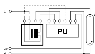
Ballasts with two tapping points and two voltage tapping points (L ST = 0 V or L ST > 0 V)
