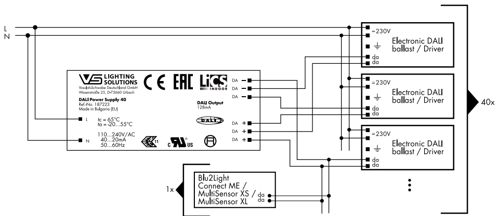
Circuit Diagram of the DALI Power Supply 40
