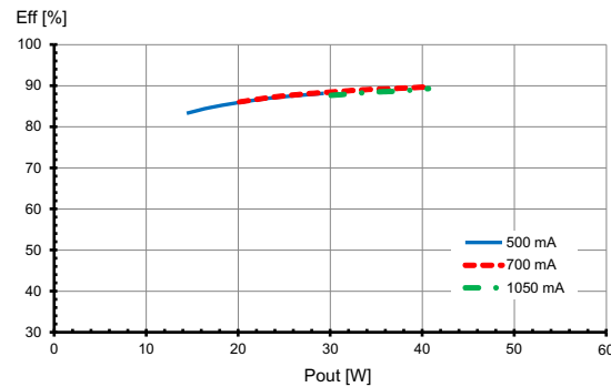
Efficiency
