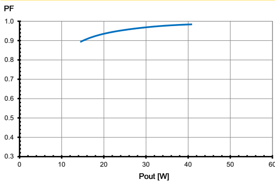
Power factor
