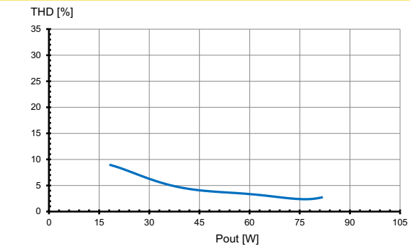
Total harmonic factor (THD)
