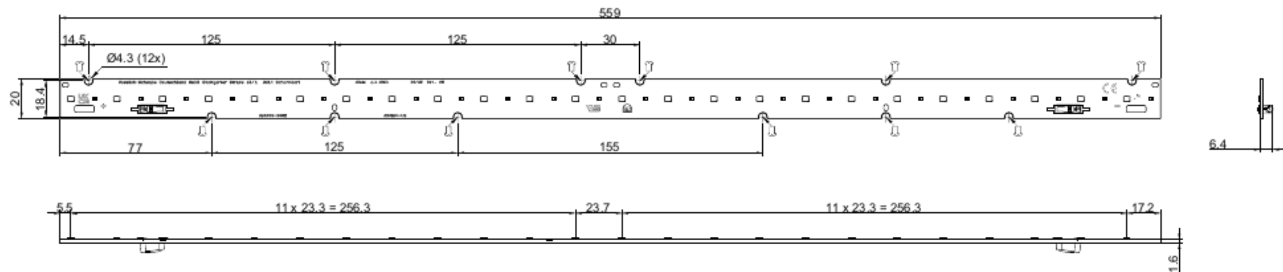
MLE SC W2/560 B/24R/yyz G3
