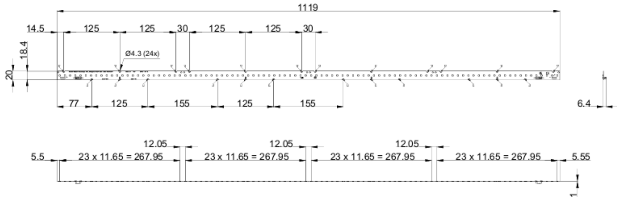
MLC SC W2/1120 B/96/yzz G3
